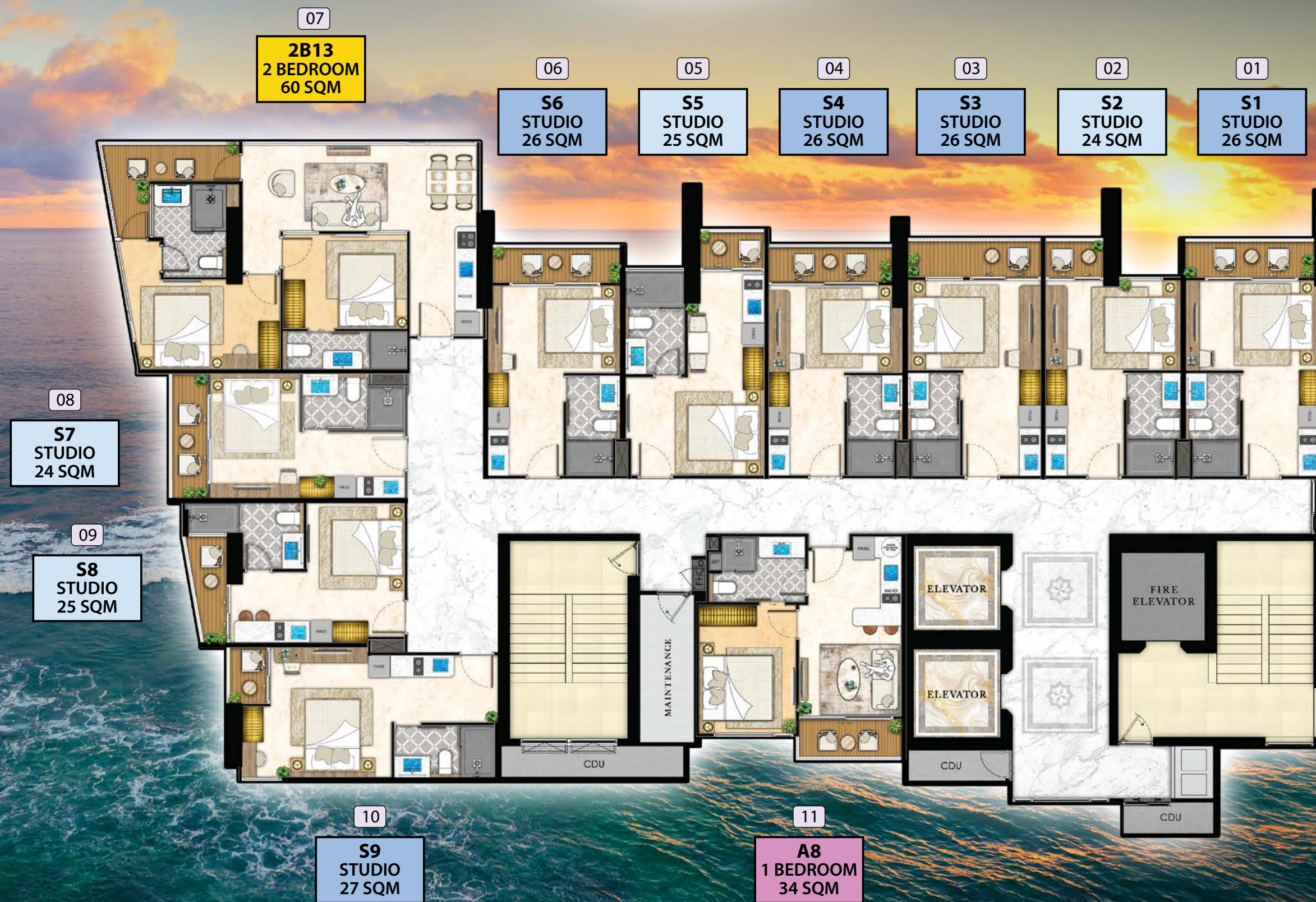
8th Floor Plan
