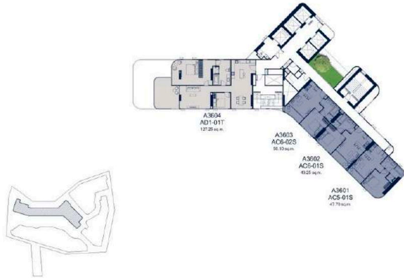
36 TH FLOOR PLAN
