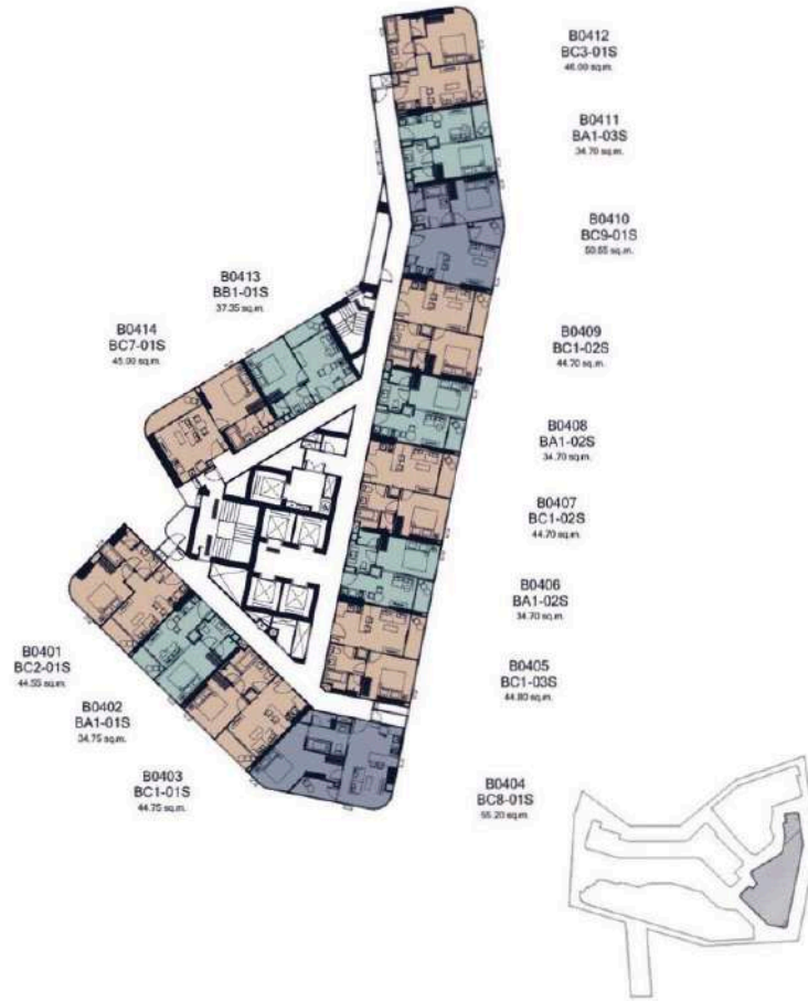
4 TH - 14 TH FLOOR PLAN
