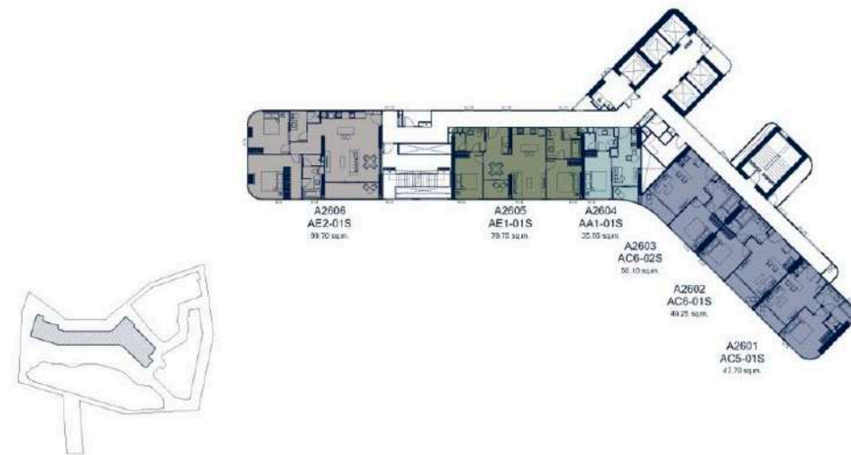
26 TH - 28 TH FLOOR PLAN
